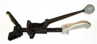
Model : OV-BHP-2532 Type : Push type Tensioner Strap Width : 19.0mm(3/4") to 32.0mm(1 1/4") Strap Thickness : 0.6mm(0.31") to 1.2mm(0.047")
