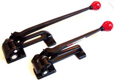
Model : OV- EFT-190 Type : Feed Wheel Type Tensioner Strap Width : 13.0mm(1/2") to 19.0mm(3/4")
