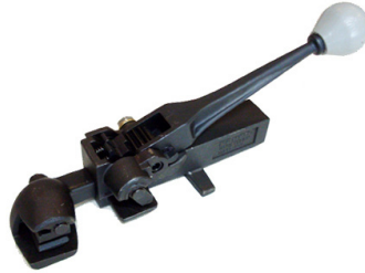
Model : OV- BTS-19 Type : Rack & Pinion Type Tensioner Strap Width : 13.0mm(1/2") to 19.0mm(3/4") Strap Thickness : 0.4mm(0.015") to 0.8mm(0.031")
